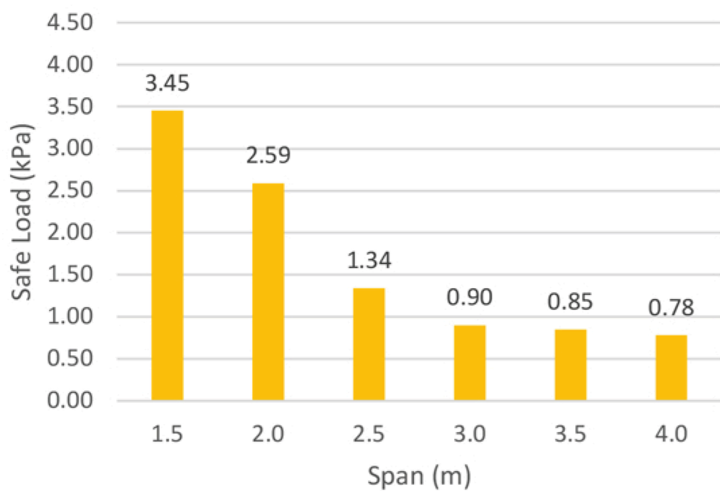
SupaPanel System with 1.15 BMT Track Safe Load (kPa) Improved-Performance Track
