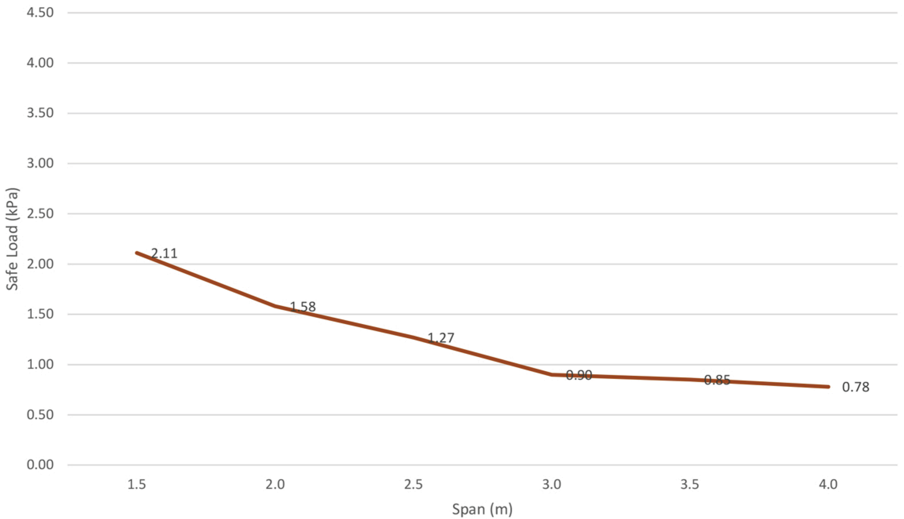
SupaPanel System with 0.9 BMT Track Safe Load (kPa) Standard Track
