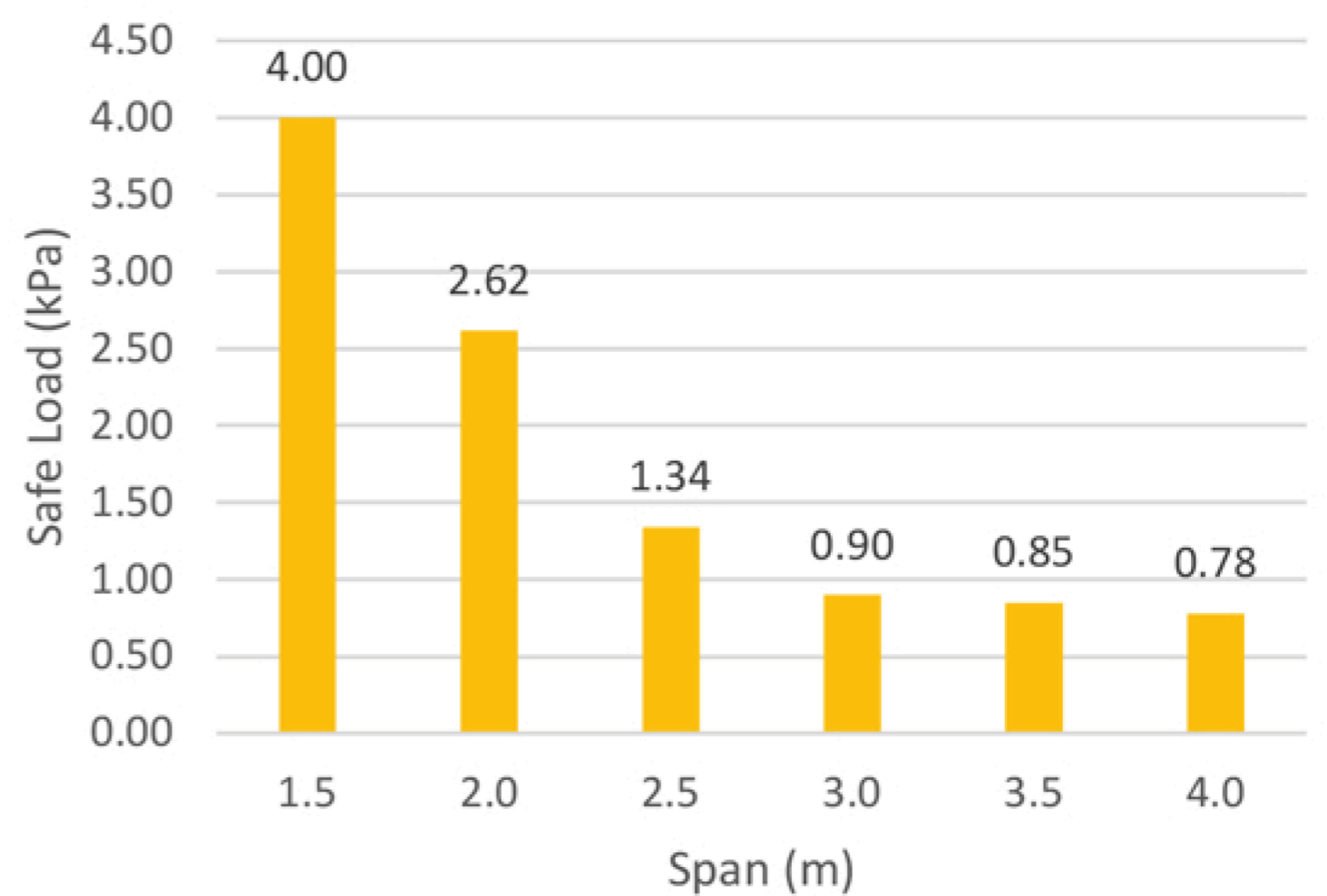
SupaPanel System with 1.5 BMT Track Safe Load (kPa) Structural Track
